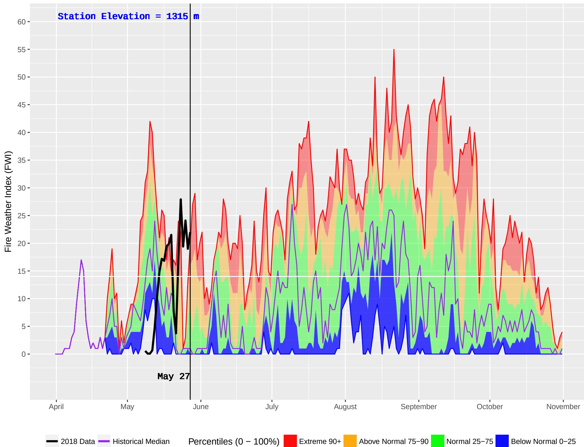
MAYSON (1082) : Historical (2010–2016) and Current (2018) Noon Fire Weather Index (FWI)
